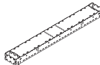
4x FLOOR S-1 (16)
